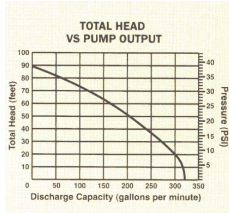
Honda WT30 3" trash pump
